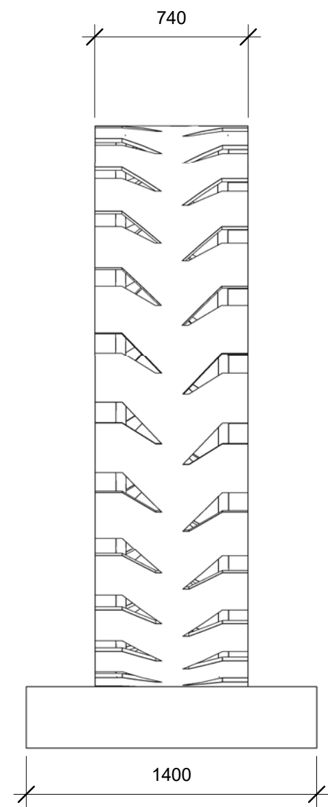
SIDE VIEW
