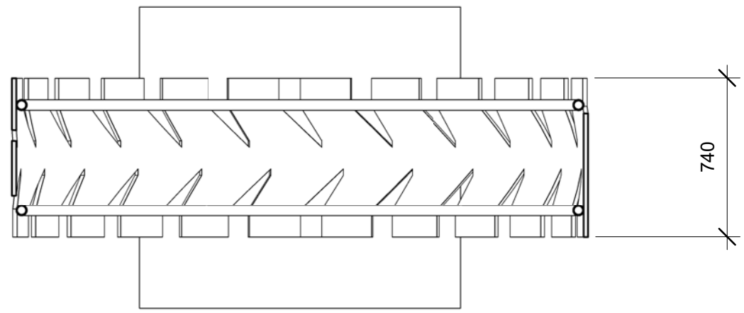
PLAN VIEW
