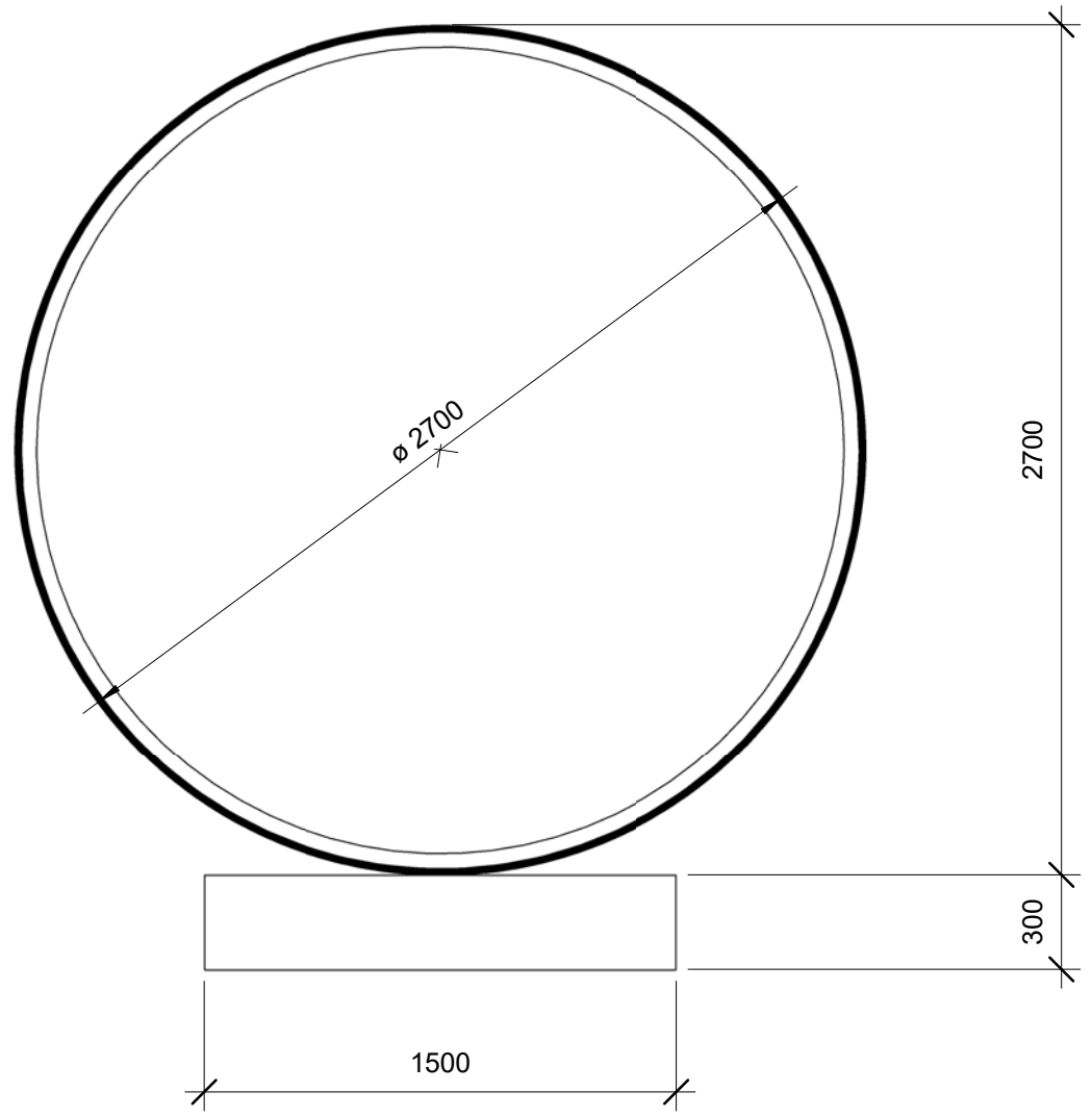
FRONT VIEW
